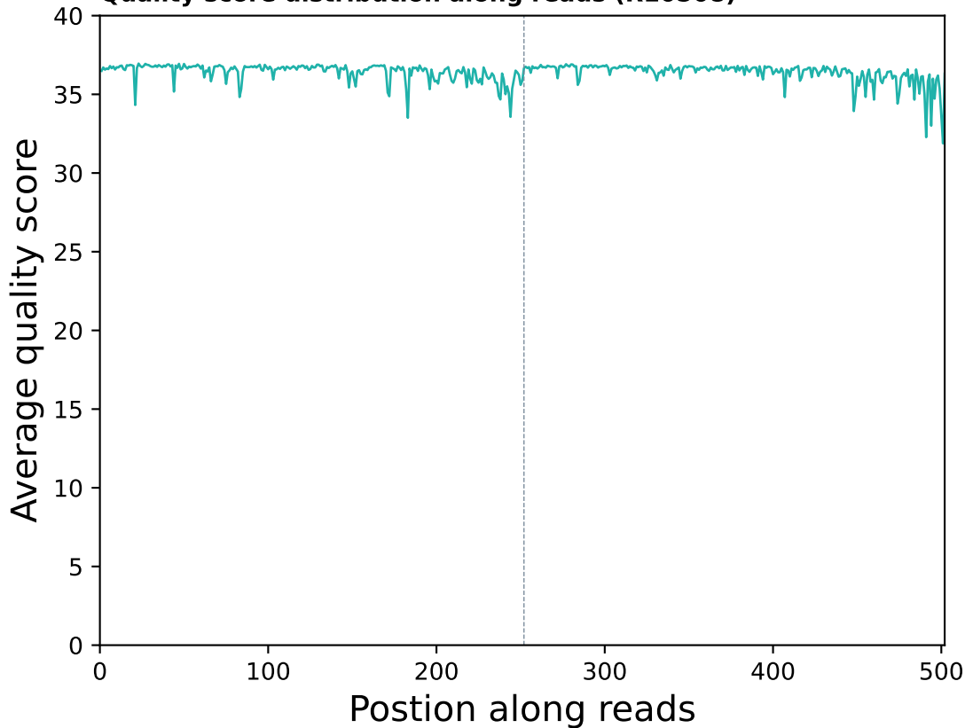
Quality score distribution along reads (R10508)
